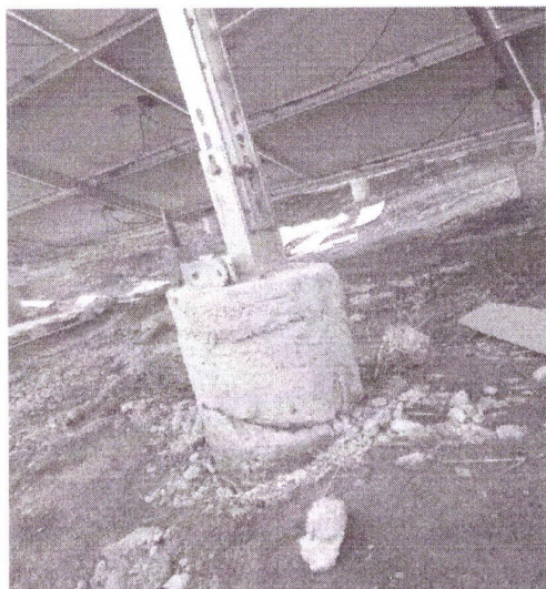
断裂的桩基基础
