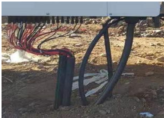
13、线管安装不规范
