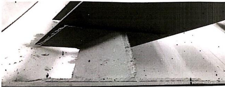
预埋高强螺栓杆生锈
