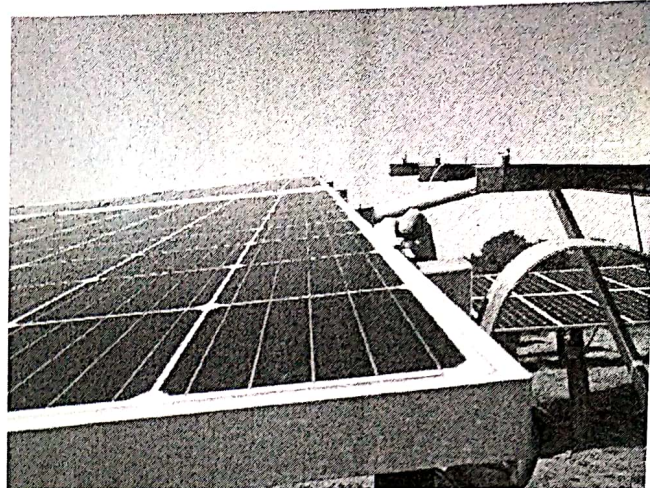
组件压块安装未紧固
