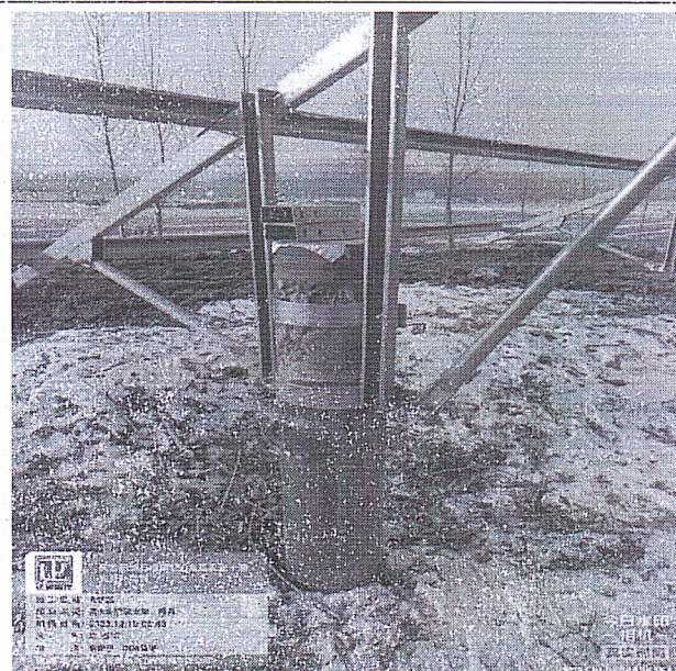
桩头损坏
