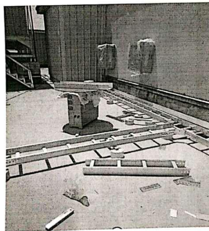
3号楼逆变器上墙安装不牢靠
