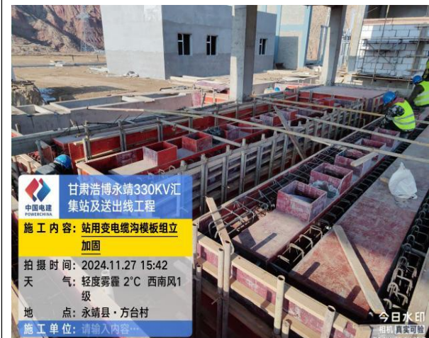
汇集站电缆沟施工
