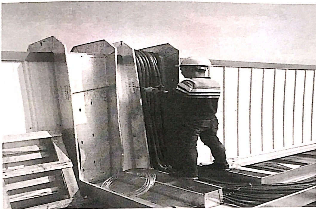
4#屋面光伏区下墙桥架电缆绑扎
