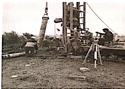
护筒埋设
